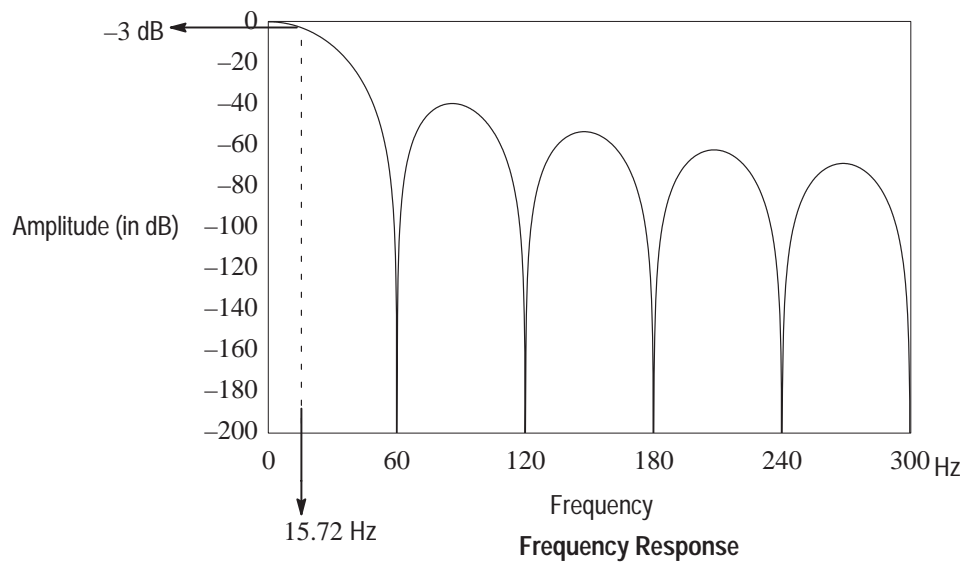
Figure 4.5 250 Hz Filter Notch Frequency
