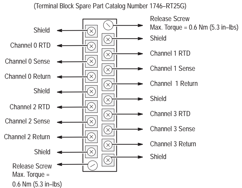
Figure 3.3 Terminal Block
