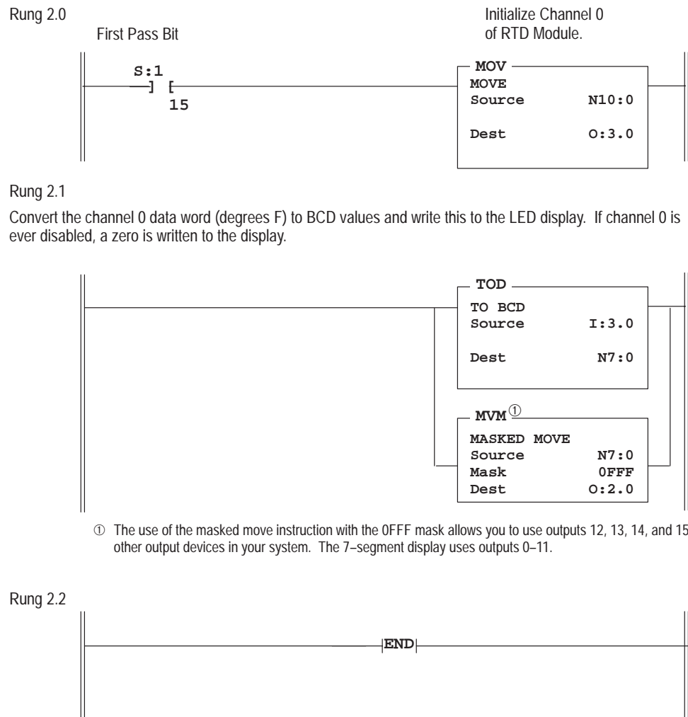
Figure 8.3 Program to Convert °F to BCD
