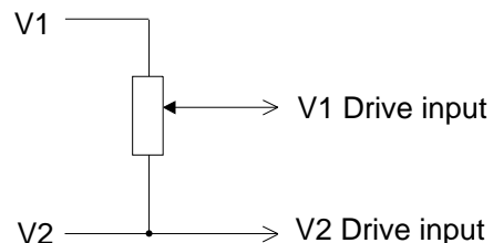
Figure 3-6. Circuit for accurate torque amp gain setting
